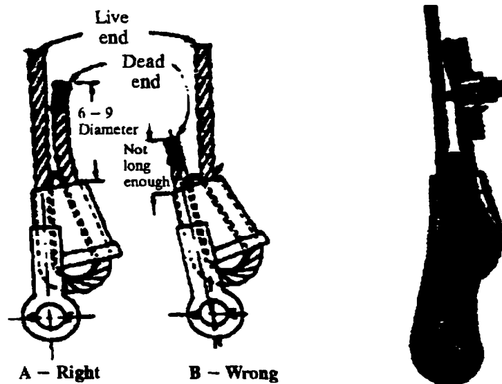
Figure C-7. Wedge Sockets
